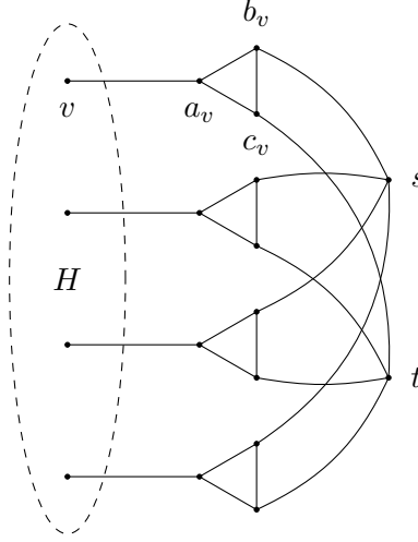
Figure 3: The graph \tilde{H} .
