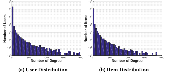
Figure 2: The distributions of users and items over different degrees in the Amazon dataset.
