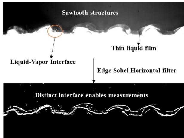
Figure 11 Liquid-vapor interface of a sliding vapor slug in FC-72 in a downward-facing orientation at 2.5 W/cm 2 . When an edge filter is applied to the backlit, contrasted image, the interface comes into sharp focus to enable measurements. (1280x800, 700 fps)
