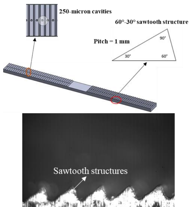
Figure 2 Details of additively manufactured test surfaces with differing sawtooth structures and 250 \mu m cavities (top). High-speed frame showing the microstructure in focus (bottom)
