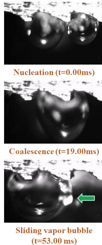
Figure 10 Sequence of images showing bubble nucleation, coalescence and sliding across the microstructure (from left to right) on a 75°-15° sawtooth in the downward-facing orientation (1280x800, 1000 fps)
