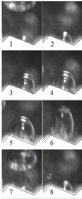
Figure 9 Series of images showing bubble nucleation and departure from a 250 \mu\text{m} cavity on a 60°-30° sawtooth (outlined in black) Frames 1-4 show the initial stages of bubble growth with a lateral component due to the surface microstructure. Frames 5-8 show the later stages of bubble growth and departure where the buoyancy forces dictate the departure direction. Bubble lifecycle was recorded over \sim 24 ms. (1280x800, 1000fps)
