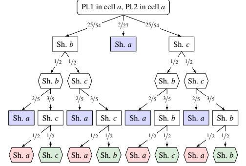
Figure 1: (Left) Probabilities of players sinking their opponent when the players play according to the SW-maximizing EFCE. For \gamma \geq 2 , the probability of the game ending with no sunken ship and the probability of Player 2 sinking Player 1 coincide. (Right) Example of a playthrough of Battleship assuming both players are recommended to place their ship in the same position a . Edge labels represent the probability of an action being recommended. Squares and hexagons denote actions taken by Players 1 and 2 respectively. Blue and red nodes represent cases where Players 1 and 2 sink their opponent, respectively. The Shoot action is abbreviated ‘Sh.’.
