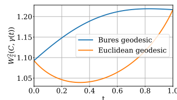
Figure 1: Example of the non-geodesic convexity of W_2^2 . Details are given in Appendix B.2.
