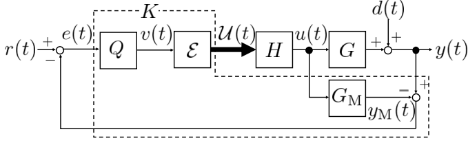
Fig. 3. Block diagram of controller K
