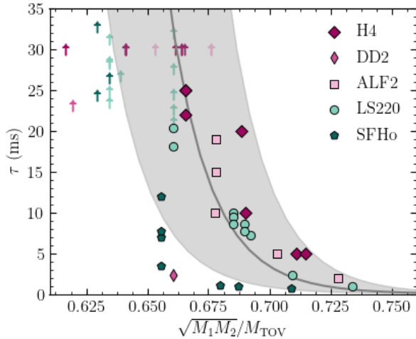
Figure 4. Lifetime of the HMNS remnant before it collapses into a black hole (if at all) as a function of \sqrt{M_1 M_2} / M_{\text{TOV}} . Up arrows indicate the HMNS survived longer than the simulation time.
