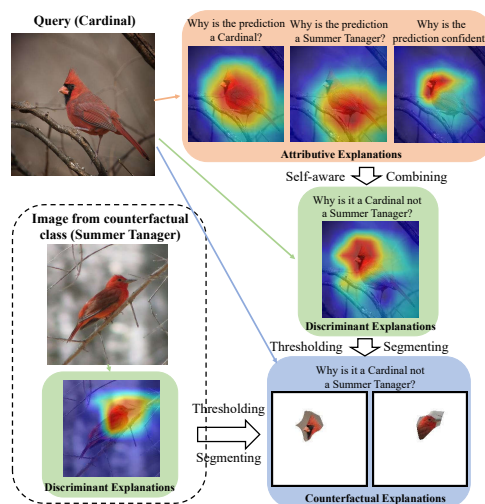
Figure 1: Given a query image (Cardinal) and a counterfactual class (Summer Tanager), discriminant explanations bridge the gap between attributions and counterfactual explanations. This enables a fast optimization-free computation of the latter.
