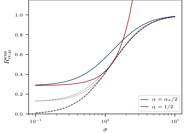
Figure 4: \mu -scaled large-ensemble risk (theoretical, \gamma = 0.5 ) when using \mu = 1 (solid) and \mu = \mu_* (dotted). For both the setting where we use fewer features than optimal with \alpha = \alpha_*/2 (blue) and the fixed \alpha = 1/2 setting (red), we see significantly improved risk by scaling.
