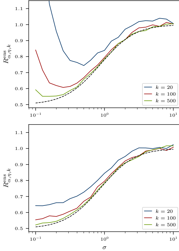
Figure 3: Approximate limiting risk (averaged over 100 trials with n = 200, p = 400 ) when using \alpha = \alpha_* (top) and \alpha = \arg \min_{\alpha'} R_{\alpha', \eta, k}^{ens} (bottom). As k increases, in both cases the risk converges to the theoretical optimal ridge regression risk (black dashed).
