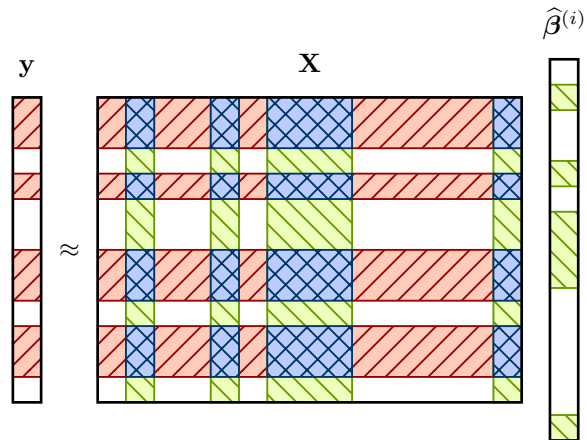
Figure 1: Example (rows) and feature (columns) subsampling of the training data used in the ordinary least squares fit for one member of the ensemble. The i -th member of the ensemble is only allowed to predict using its subset of the features (green). It must learn its parameters \hat{\beta}^{(i)} by performing ordinary least squares using the subsampled examples of y (red) and the subsampled examples (rows) and features (columns) of the data matrix X (blue, crosshatched).
