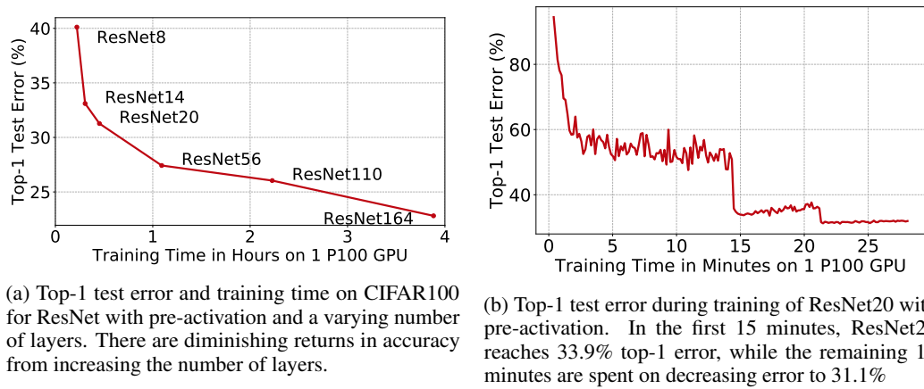
Figure 5: Top-1 test error on CIFAR100 for varying model sizes (left) and over the course of training a single model (right), demonstrating a large amount of time is spent on small changes in accuracy.
