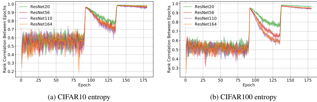
Figure 14: Average ( \pm 1 std.) Spearman's rank-order correlation between epochs during 5 training runs of varying ResNet architectures on CIFAR10 (left) and CIFAR100 (right), where rankings were based on entropy.
