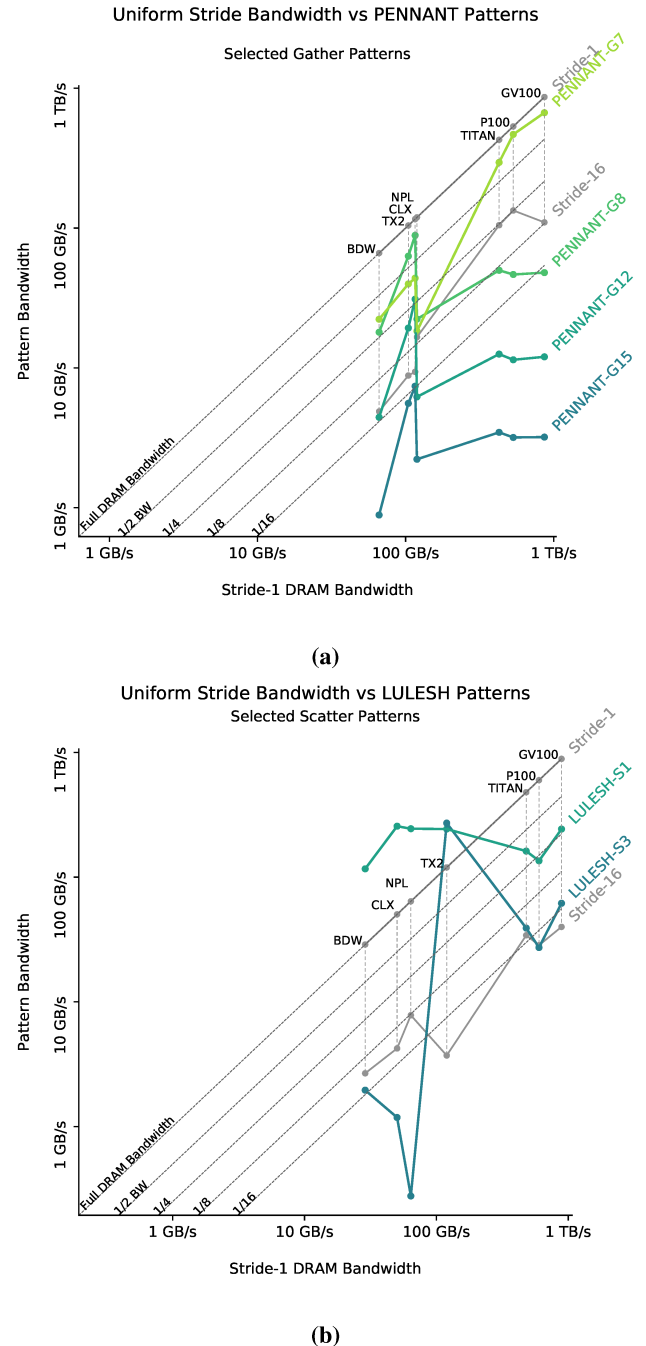
Figure 9: Bandwidth-Bandwidth Plots
