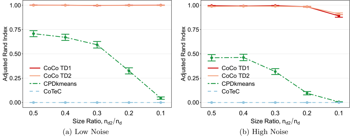
Figure 6: Checkbox Simulation Results: Impact of Cluster Size Imbalance. Two imbalanced clusters per mode with either low or high homoskedastic noise for n_1 = n_2 = n_3 = 60 . Low noise corresponds to \sigma = 3 while high noise refers to \sigma = 6 .
