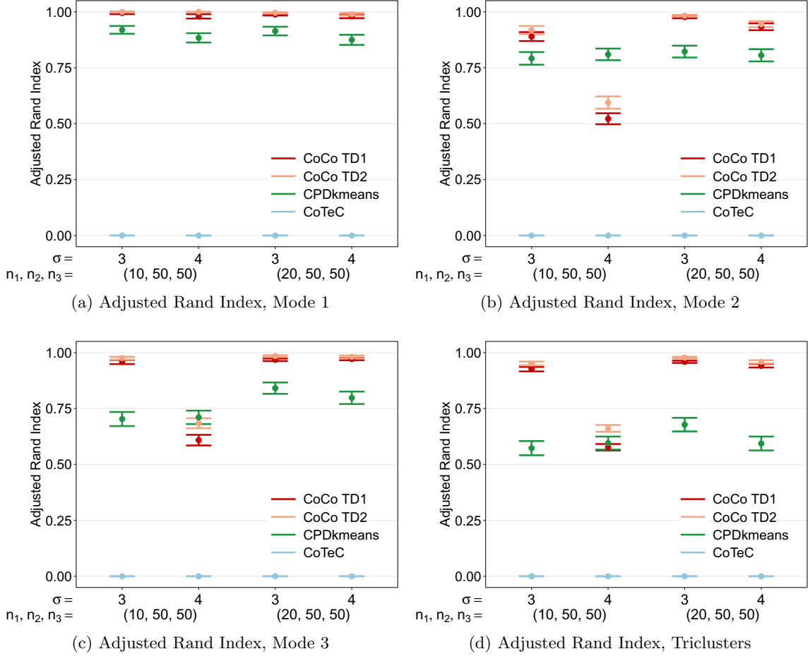
Figure 9: Checkbox Simulation Results: Impact of Tensor Shape. Two balanced clusters per mode with two levels of homoskedastic noise for a tensor with one short mode and two longer modes. Average adjusted rand index plus/minus one standard error for different noise levels and mode lengths.
