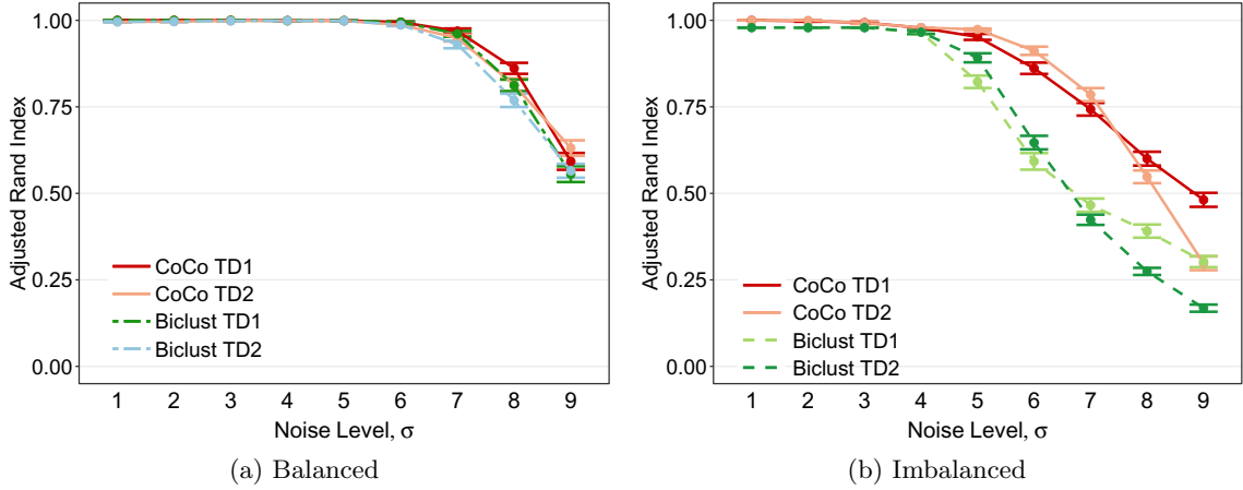
Figure 12: A Comparison between CoCo and Convex Biclustering Average Adjusted Rand Index plus/minus one standard error for different noise levels.
