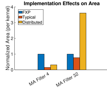
Figure 4. Effects of implementation details on area. “Typical” designates a stochastic bitstream design of Eq. 4 and “Distributed” designates a stochastic bitstream design of Eq. 5. In the latter case, the bitstream design consumes more area than the FXP design for an 32-wide MA filter.
