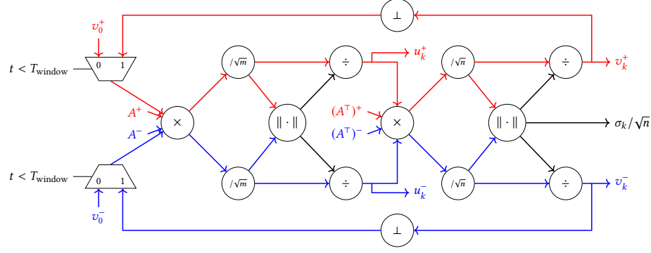
Figure 3. A block diagram of the bitstream computing iterative SVD. T_{\text{window}} is the window length over which we estimate a stochastic bitstream. The /x blocks denote a fixed gain division by x , the \perp blocks denote a decorrelator, and the \| \cdot \| blocks denote the L2-norm. [6] and [11] provide details on the implementations of these blocks. Red denotes positive channels and blue denotes negative channels for signed compute as detailed in [6].
