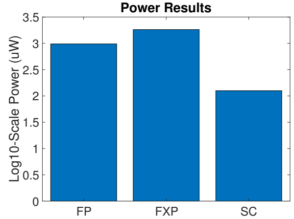
Figure 7. Total power results for floating point (FP), fixed point (FXP), and stochastic computing (SC) designs when mapped to a Lattice LM4K FPGA (note y-axis is log-scale). The SC design is an order of magnitude lower power than the traditional designs.
