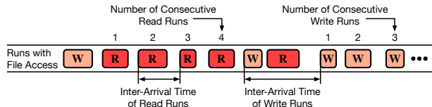
Figure 4: Visual representation of inter-arrival times and number of consecutive runs for both read (R) and write (W) runs.
