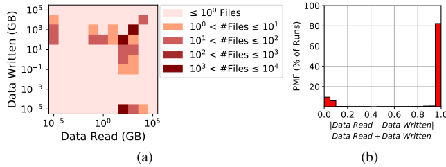
Figure 3: (a) Files can be divided into groups: read-heavy (RH), write-heavy (WH), or both, read- and write- heavy (RW). (b) Difference in data read and written per run shows > 82\% of runs either perform only read I/O or only write I/O.
