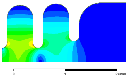
Figure 4: Normalized electric field distribution for the TM_{01} \pi -mode. The maximum field on axis is 706 MV/m and the peak surface field is 1.18 GV/m.
