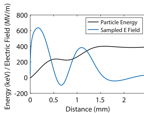
Figure 5: Sampled on-axis electric field (blue) and the resulting change in electron energy (black) for 1 MW of input gyrotron power and a launch phase of 60 degrees.
