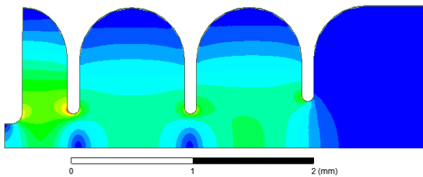
Figure 2: Normalized electric field distribution for the TM_{01} \pi -mode. The maximum field on axis is 838 MV/m and the peak surface field is 1.86 GV/m.
