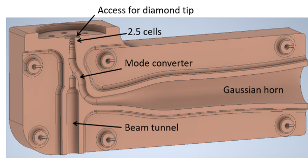
Figure 6: Model of one half of the split-block 2.5 cell prototype. The diamond tip substrate will be attached to the top of the block when the two halves are assembled. The cells, mode converter, Gaussian horn, and electron beam tunnel are indicated.
