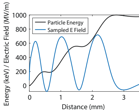
Figure 3: Sampled on-axis electric field (blue) and the resulting change in electron energy (black) for 2.75 MW of input gyrotron power and a launch phase of 60 degrees.
