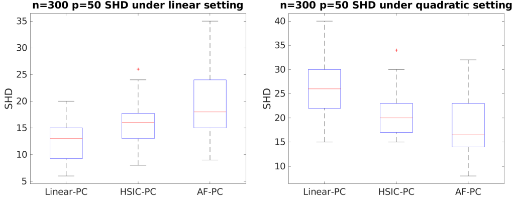
Figure 4: Boxplots of \text{SHD}(\hat{\mathbf{E}}_{\text{CPDAG}}) from AF-PC, HSIC-PC, and linear-PC.
