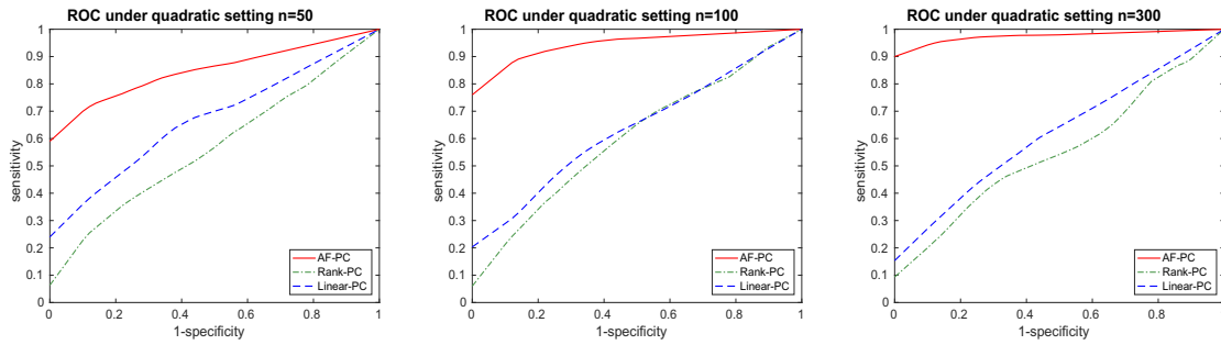
Figure 3: Comparisons of the ROC curves by AF-PC, rank-PC, and linear-PC on quadratic models.
