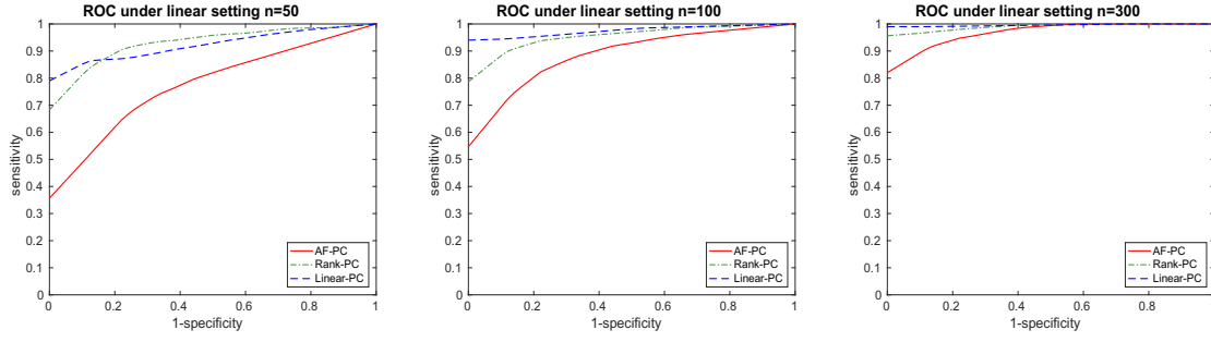
Figure 2: Comparisons of the ROC curves by AF-PC, rank-PC, and linear-PC on linear models.
