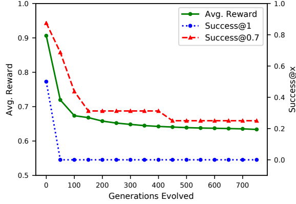
Figure 4. Performance of the best heuristic model on packs that are evolved to a varying extent. The left-hand y-axis is for Avg. Reward and the right-hand y-axis is for the Success@x metrics. The performance of the best heuristic decreases with evolution showing that the packs become more challenging with evolution.
