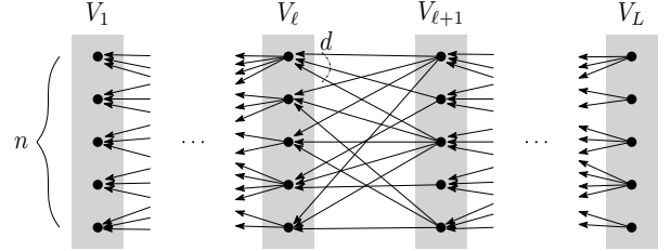
Figure 3. The figure shows the DAG with L layers V_1, \dots, V_L representing the nL jobs. Each of the n jobs in V_\ell has dependencies on d randomly chosen jobs in V_{\ell+1} . We set \rho = d^L , m = \rho , and the parameters L = c_1 \sqrt{\log n} , d = 2^{c_2 \sqrt{\log n}} for some appropriate constants c_1, c_2 > 0 .
