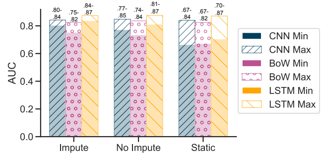
Figure 1: This plot reports the best (max) and worst (min) AUC scores across all embeddings for each model on the OLID dataset. The exact range (Min-Max) is shown above each bar.
