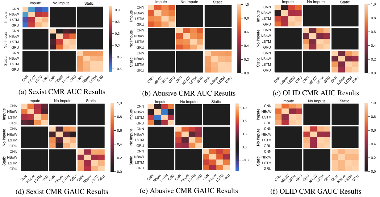
Figure 2: Cross-Model Reliability (CMR) correlation heatmap measured by the Spearman rho correlation between the performance scores (AUC and GAUC) of different models trained on the same dataset. The correlation measures whether the word embeddings that result in the best (worst) performance for a given model are the same for different models.
