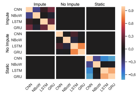
Figure 3: Abusive Cross-Model Reliability (CMR) FPED Results.
