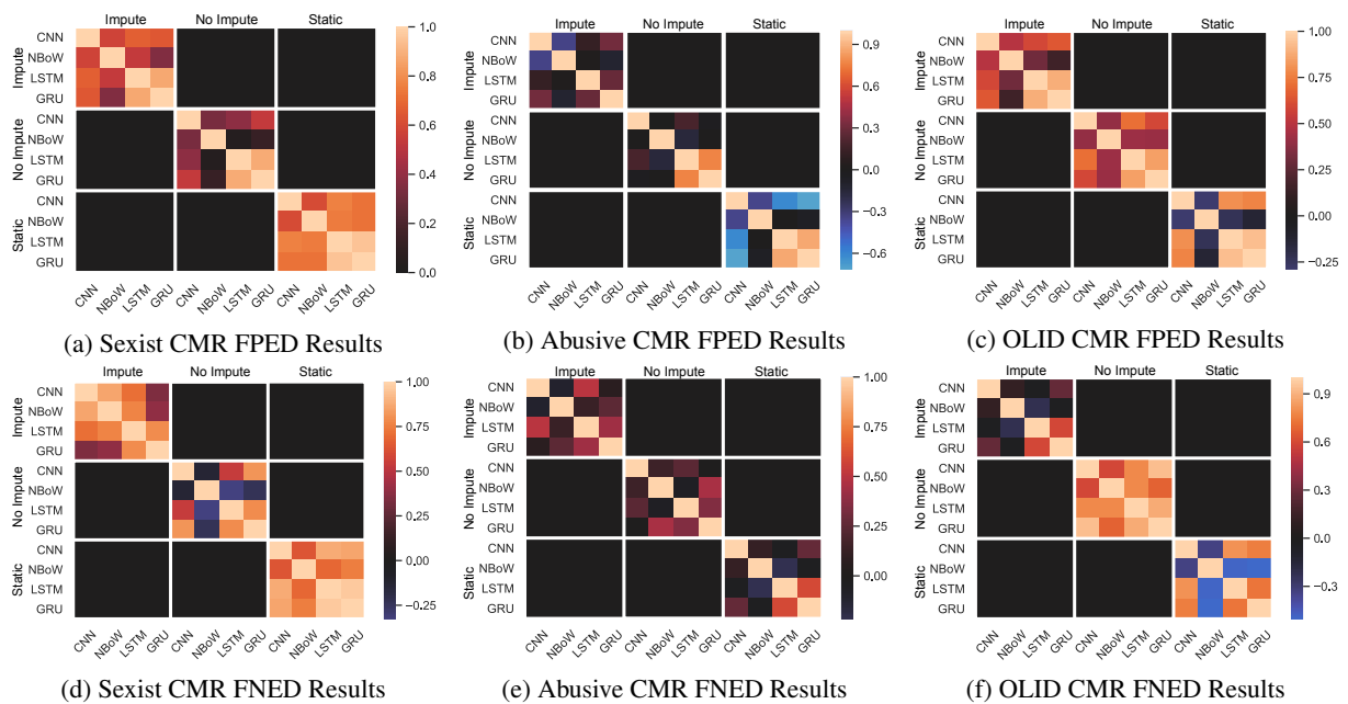
Figure 4: Cross-Model Reliability (CMR) correlation heatmap measured by the Spearman rho correlation between the performance scores (FPED and FNED) of different models trained on the same dataset. The correlation measures whether the word embeddings that result in the best (worst) performance for a given model are the same for different models.
