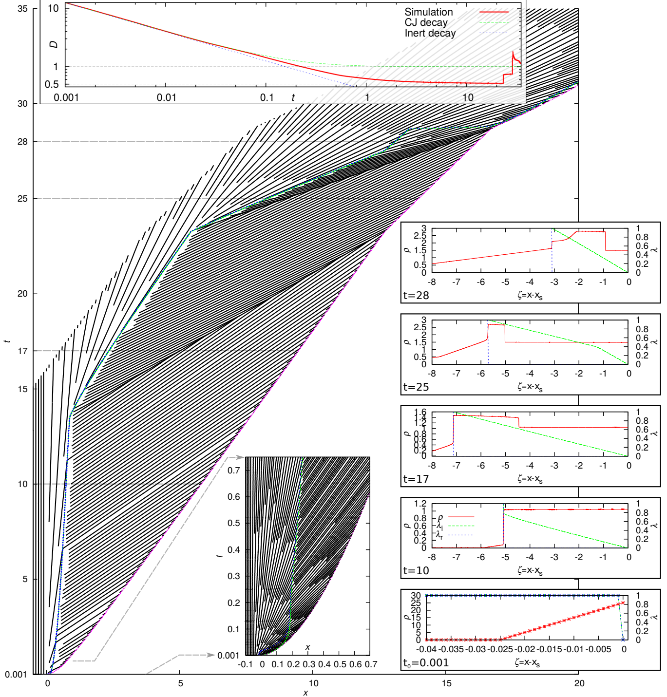
Figure 2: Characteristics diagram in the lab frame of reference ( -9 \leq x - x_s \leq 0 ) with characteristics in black, the shock front in magenta, the ends of the induction and reaction zones in green and blue, and particle paths that follow vertical lines (along which reactions take place, not shown); a magnification of early times is centred at the bottom; insets show profiles of \rho and \lambda on the right and blast speed at the top, see insets for their legends; ( E_b = 5/32 , E_a = 5.5 , k = 100 ; ostensibly similar to the subcritical case of figure 1, with more distinct features and shorter scales)
