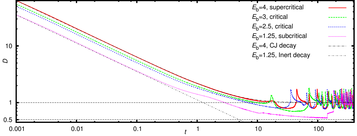
Figure 1: Numerical solutions for three different blast energies yielding supercritical and critical detonation initiations, and the subcritical case (detonation failure); inert and CJ blast decays shown for lowest blast energy case; horizontal dashed lines placed at D_{CJ} = 1 and D_{CJ}/2 ; ( E_a = 10 , k = 5 )
