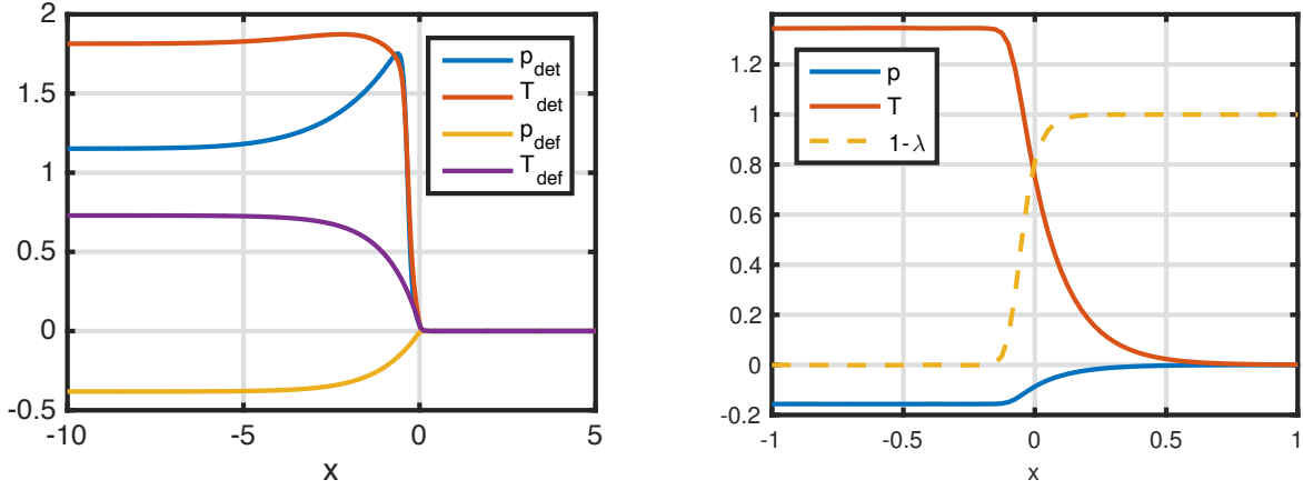
(a) Supersonic and subsonic traveling wave solutions of (8)–(10) with \mathcal{M} \approx 1 . The dominant balance is between advection and reaction. (b) Traveling wave solution of (11)–(13) with \mathcal{M} \ll 1 . Diffusion plays an important role, and the pressure drops across the wave.
