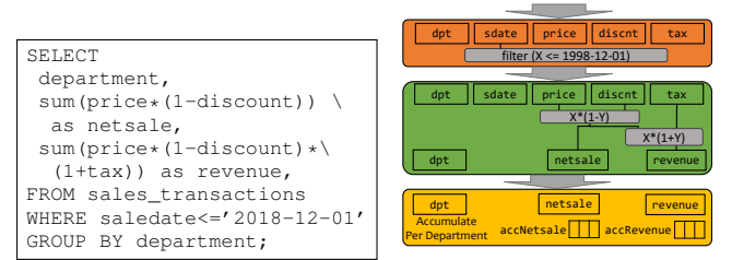
Fig. 1: Dataflow of an Aggregate Query
