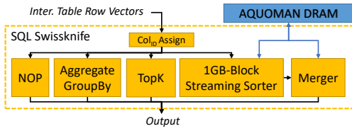
Fig. 11: SQL Swissknife Architecture
