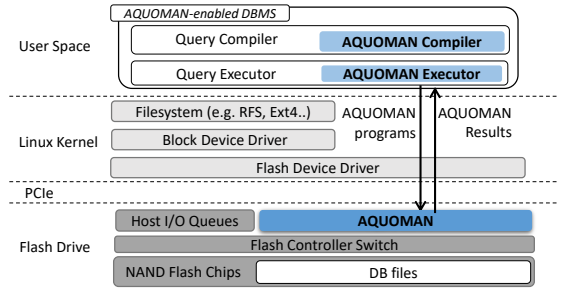
Fig. 3: System Stack with AQUOMAN
