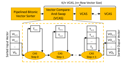
Fig. 13: TopK Accelerator
