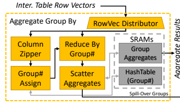
Fig. 12: Aggregate-GroupBy Accel.
