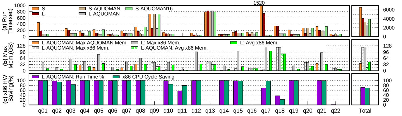
Fig. 16: TPC-H SF-1000 AQUOMAN Performance Profiling
