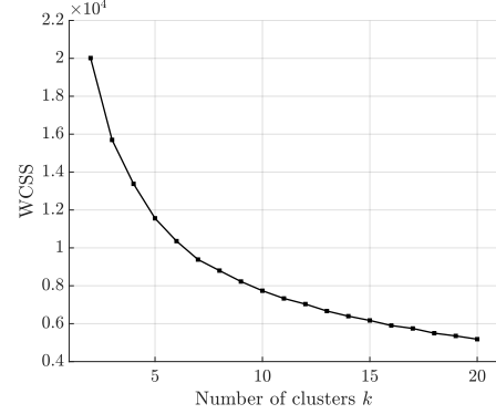
Fig. 6. Within cluster sum-of-square (WCSS) error versus the number of clusters.
