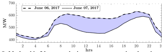
Fig. 8: Netload in Vermont during two consecutive days in summer.
