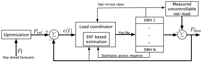
Fig. 1: Closed-loop feedback system for PEM with P_{\text{ref}} provided by the grid or market operator and the aggregate net-load P_{\text{dem}} measured by the coordinator.
