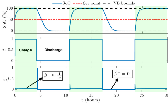
Fig. 2: SoC during a 30 hour dis/charging simulation showing a first-order response. Highlighted region shows PEM-VB charging.
