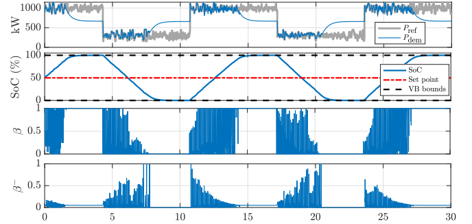
Fig. 4: Tracking when reaching upper and lower energy boundaries. System is unable to track once energy limits are reached.
