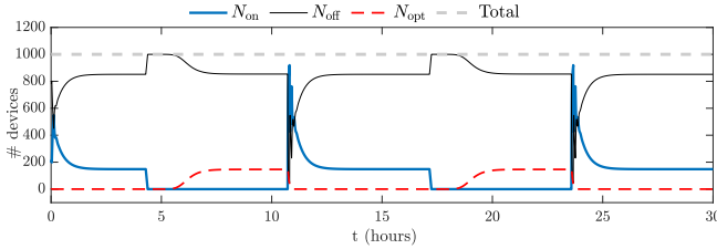
Fig. 3: N_{\text{on}} , N_{\text{off}} and N_{\text{opt}} during a 30 hour charging/discharging simulation. The total number of devices is always preserved.
