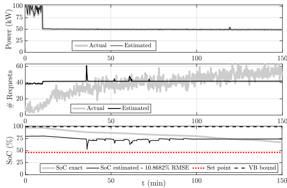
Fig. 7: Estimating SoC while tracking a reference without x_r .
