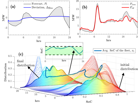
Fig. 9: Optimal dispatch of EWHs. (a) Net load forecasts ( P_f ) and setpoint of generators ( g ), (b) nominal power consumption, P_{\text{nom}} and the input P_{\text{ref}} , (c) evolution of EWHs SoC distribution. PEM-VB captures the average SoC or energy of the fleet. The Kullback-Leibler divergence between initial and final distributions is 0.061.
