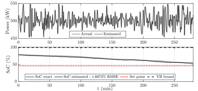
Fig. 5: Tracking an AGC signal from ISO-NE.
