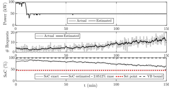
Fig. 6: Estimating SoC while tracking a reference with x_r .
