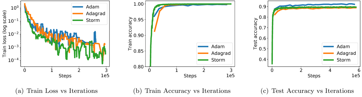
Figure 1: Experiments on CIFAR-10 with ResNet-32 Network.
