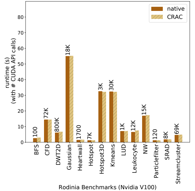
Fig. 2: Runtimes of 14 Rodinia benchmarks with total CUDA API calls made by each benchmark (rounded off)
