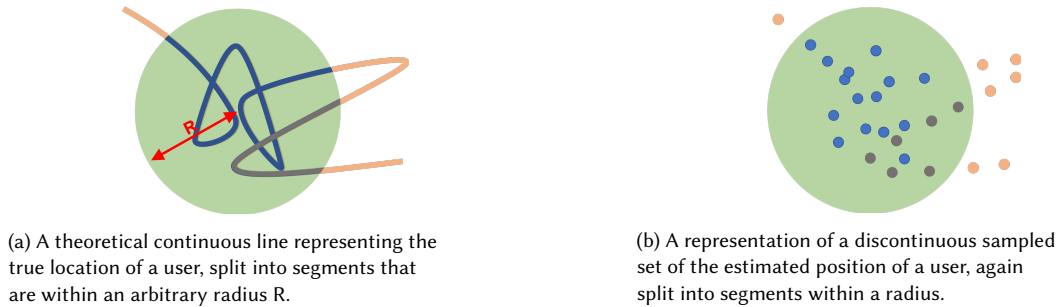
Fig. 2. Theoretical versus discontinuous representation of position estimation.
