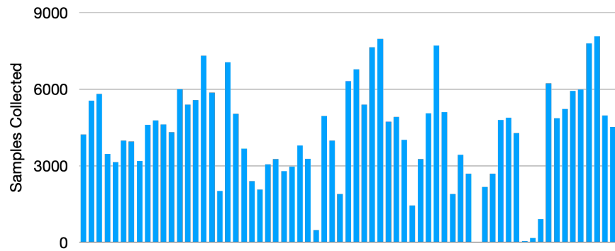
Fig. 1. Location data points aggregated by day over the course of the experiment. The number of samples collected per day varies greatly.
