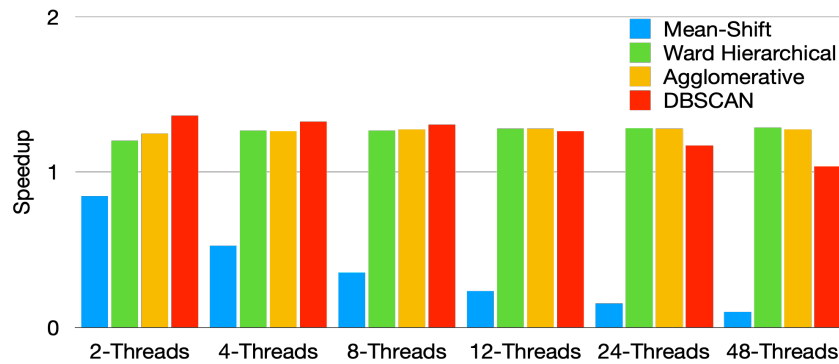
Fig. 3. Strong scaling of off-the-shelf algorithms that were trivial to add parallel functionality. Due to the extreme runtimes/memory constraints, the small dataset was used to show speedup.
