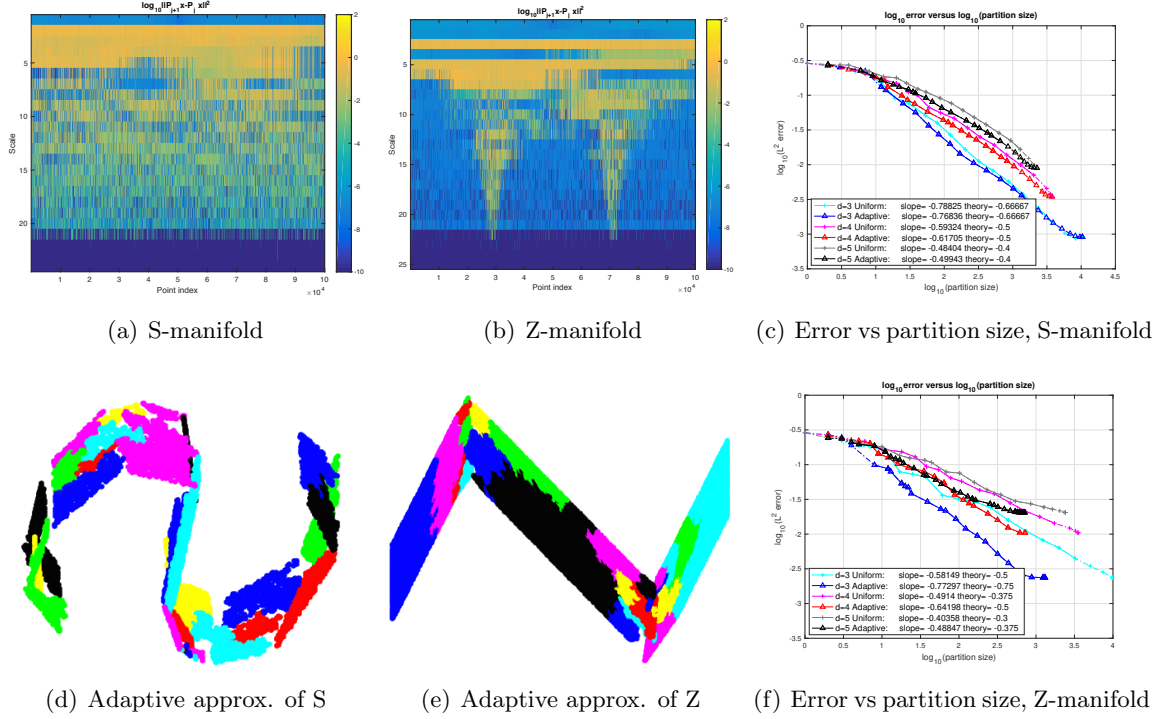
Figure 4: (a,b): \log_{10} \|\hat{\mathcal{P}}_j(x_i) - \hat{\mathcal{P}}_{j+1}(x_i)\| from the coarsest scale (top) to the finest scale (bottom), with columns indexed by points, which, for visualization purposes only, are sorted roughly from “left to right” on the manifold. (d,e): adaptive approximations: for the S-manifold the adaptive approximation is close to a uniform approximation, but for the Z-manifold it contains few large pieces near the almost-flat regions, and several small pieces near the “corners”. (c,f): log-log plot of the approximation error versus the partition size in GMRA and Adaptive GMRA respectively. Theoretically, the slope is -2/d in both GMRA and Adaptive GMRA for the S-manifold. For the Z-manifold, the slope is -1.5/d in GMRA and -1.5/(d-1) in Adaptive GMRA (see appendix B).
