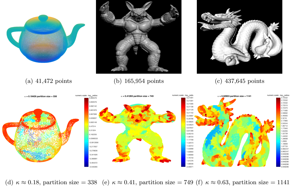
Figure 9: Top line: 3D shapes; bottom line: adaptive partitions selected with refinement criterion \hat{\Delta}_{j,k} \geq 2^{-j}\kappa\sqrt{(\log n)/n} . Every cell is colored by scale. In the adaptive partition, at irregular locations cells are selected at finer scales than at “flat” locations.
