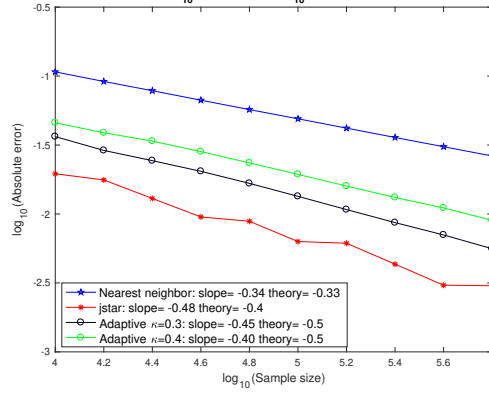
(a) the 3-dim S-manifold, \sigma = 0
