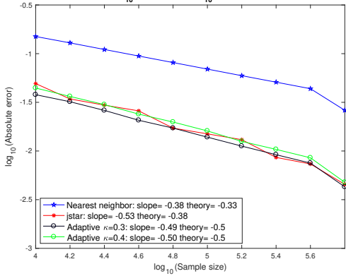
(c) the 3-dim Z-manifold, \sigma = 0
