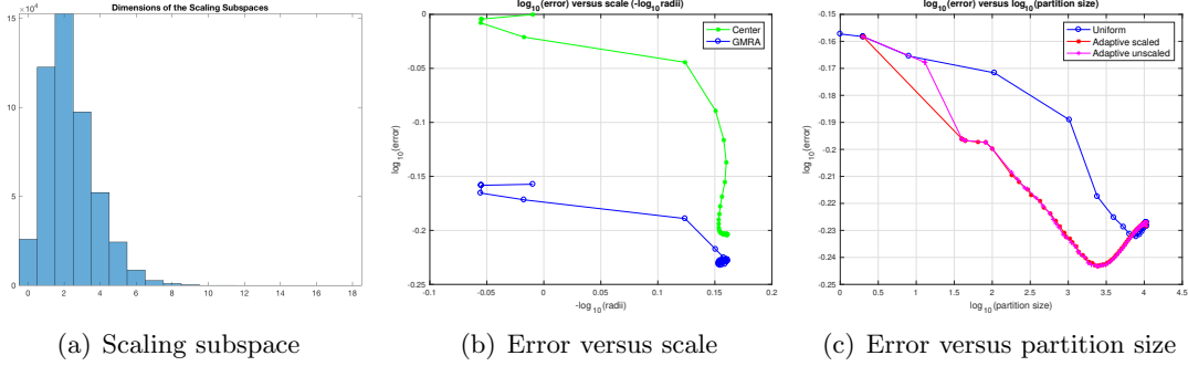
(a) Scaling subspace
