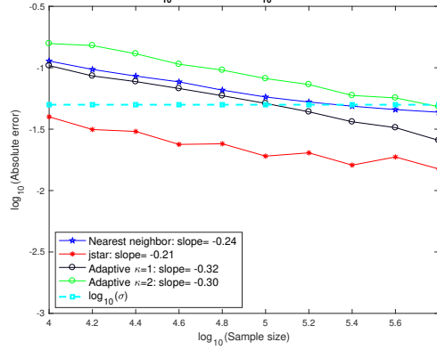
(b) the 3-dim S-manifold, \sigma = 0.05
