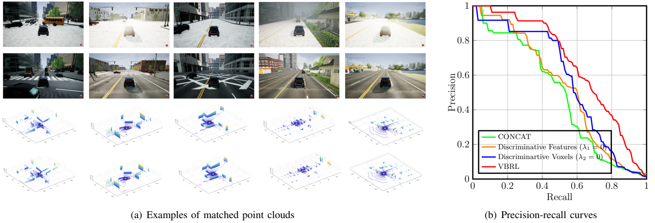
Fig. 2. Qualitative and quantitative experimental results over the AirSim simulations.
