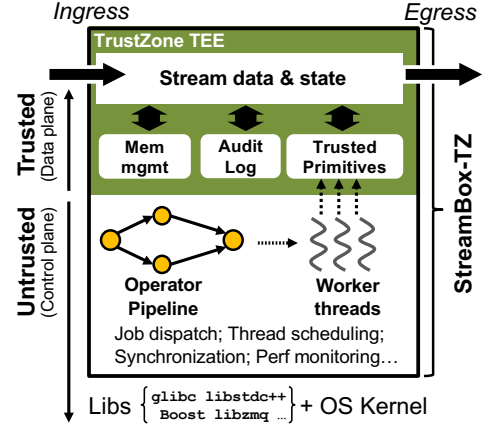
Figure 3: StreamBox-TZ on an edge platform with ARM TrustZone. Bold arrows show the protected data path.
