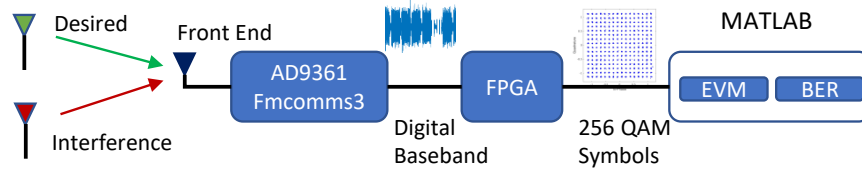
Fig. 8: EVM and BER measurement workflow. The received signal goes through analog and digital signal processing elements of the AD9361, and digital baseband operations such as synchronization and channel estimation are performed on the FPGA in real time.
