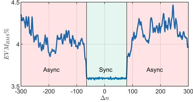
Fig. 5: Plot of percentage EVM vs \Delta n when \Delta f = 0 kHz at an SNR of 30 dB. \tau_{max-} and \tau_{max+} are 65 and 79, respectively when p = 0.55 . Note that the EVM is lowest when the interference is synchronous to the desired signal.
