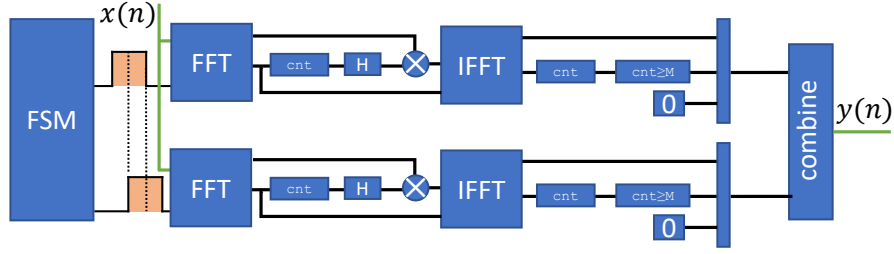
Fig. 9: Frequency domain F-OFDM filter implementation (block level).
