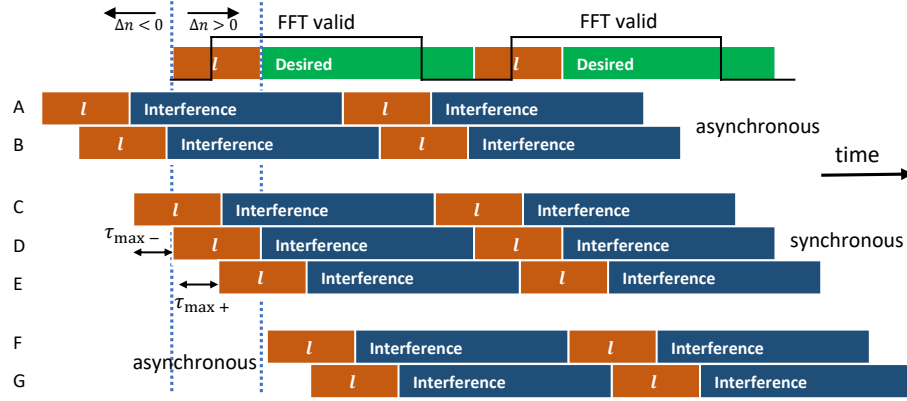
Fig. 4: Illustration of asynchronous and synchronous interference for different values of \Delta n . The letters A-G show different possible time misalignment situations of the same interference signal with respect to the desired signal. In A and B, \Delta n < \tau_{max-} , and in F and G, \Delta n > \tau_{max+} meaning that such situations are asynchronous. C, D and E satisfy Eq. (1), hence are synchronous.
