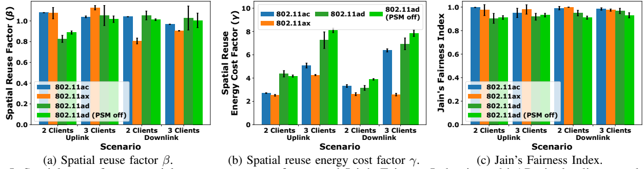
Fig. 5: Spatial reuse factor, spatial reuse energy cost factor, and Jain's Fairness Index in multi-AP, single-client topologies.
