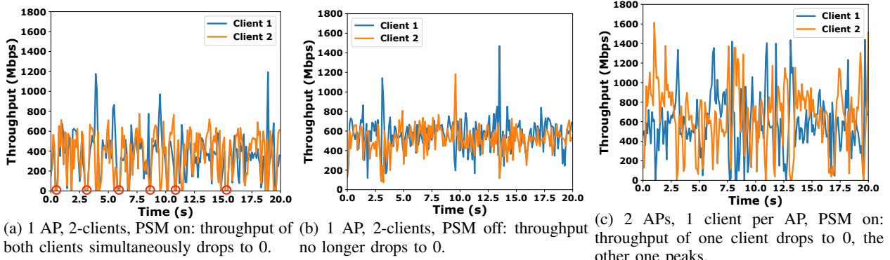
Fig. 6: Example throughput timelines in multi-client and multi-AP topologies.
