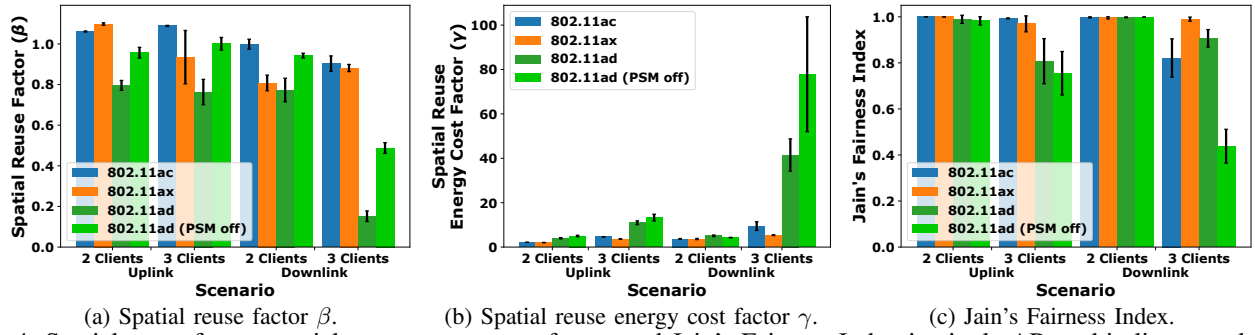
Fig. 4: Spatial reuse factor, spatial reuse energy cost factor, and Jain's Fairness Index in single-AP, multi-client topologies.
