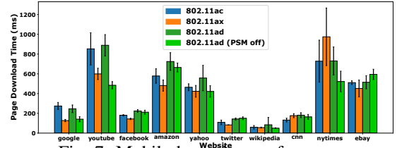
Fig. 7: Mobile browsing performance.
