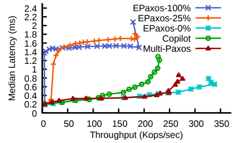
Figure 8: Throughput and latency with the thrifty optimization of the systems when there are no slow replicas.
