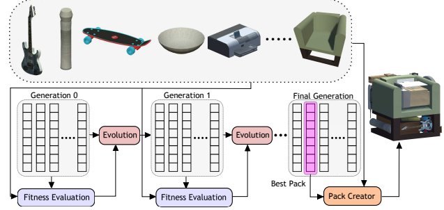
Figure 2. A schematic representation of the proposed evolutionary algorithm for generating packs. Given a pool of shapes as input, it selects a subset of shapes and appropriately scales, rotates and places them inside a unit box in order to generate high-density packs.
