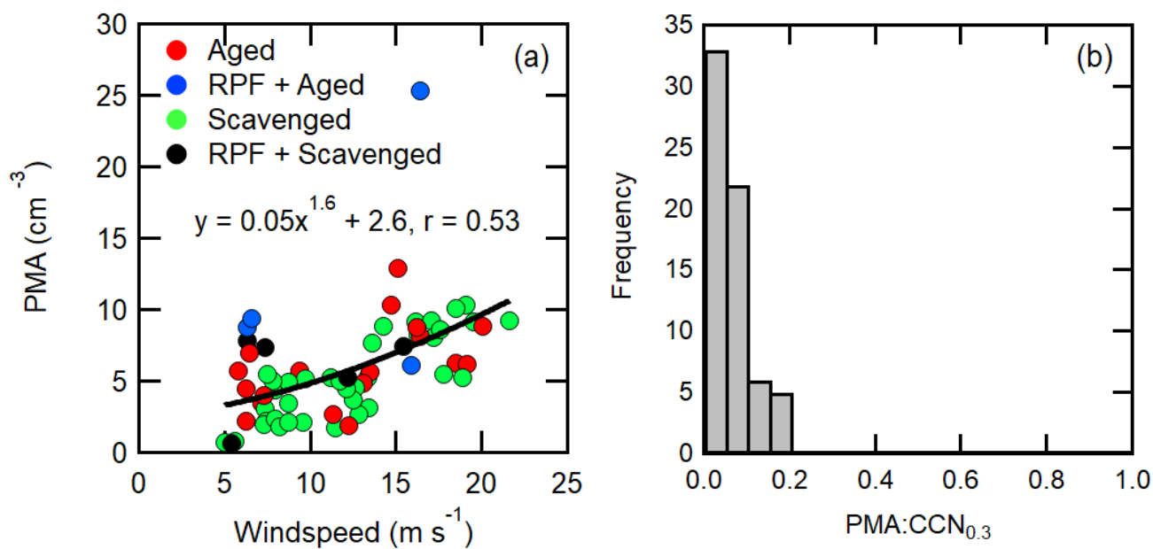
Figure 7. (a) Correlation of estimated PMA concentration and wind speed, and (b) the fraction of PMA accounting for \text{CCN}_{0.3} for MBL legs. Exclusion of the outlier in (a) increases the Pearson's Coefficient to 0.59 .
