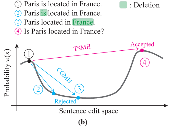
Figure 1: (a) Natural language generation via constraint satisfaction (bottom), comparing to supervised approach (up). (b) Our proposed tree search enhanced MCMC (TSMH, pink line) traverses the probabilistic space of high-quality sentences more effectively than the baseline (blue line).
