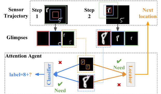
Figure 2: The unique challenge of attention-based classification with only a small number of training samples. A classifier will overfit if it learns to use the locations instead of the contents of ROIs. To prevent overfitting, a classifier should avoid “memorizing” locations in a low-resolution glimpse and focus on the high-resolution glimpse. Meanwhile, a “locator” network should utilize the low-resolution glimpse to determine where to move the sensor next.
