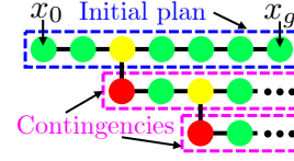
Fig. 5: Policy tree: initial plan and contingencies, rooted at possibly unsafe states. Green / red / yellow states in \mathcal{G}_s / \mathcal{G}_{\neg s} / \text{proj}_C(\mathcal{F}_\theta) .
