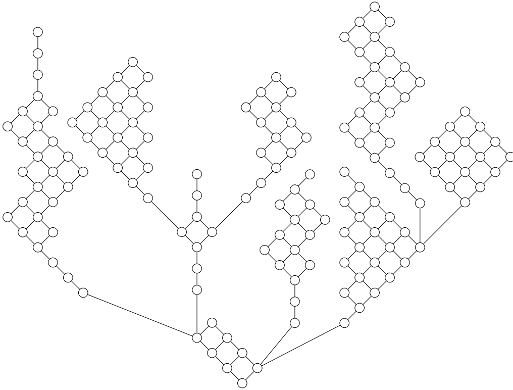
Figure 1: The Hasse diagram of a representative d -complete poset \mathcal{P} that is “built from minuscule posets” in the sense of Theorem 2. In \mathcal{P} , every order ideal \lambda \subseteq \mathcal{P} has a unique rectification target, provided by Theorem 2.
