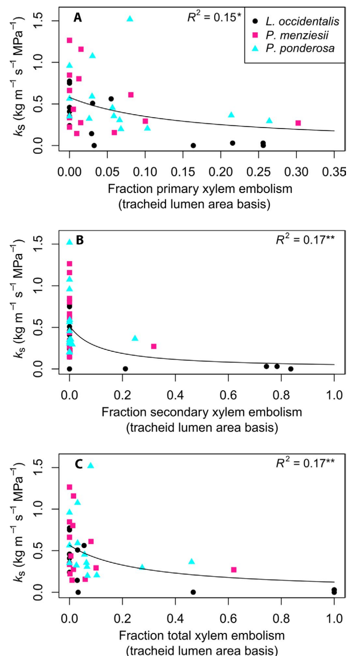
FIGURE 5. Response of conductivity broken down between tissues: (A) primary xylem embolism, (B) secondary xylem embolism, and (C) total xylem embolism. Significance of R^2 : ** 0.001 \leq P < 0.01 and * 0.01 \leq P < 0.05 .
