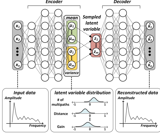
Figure 5: RF-EATS's Variational Autoencoder.
