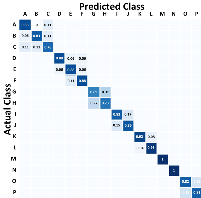
Figure 13: Confusion Matrix
