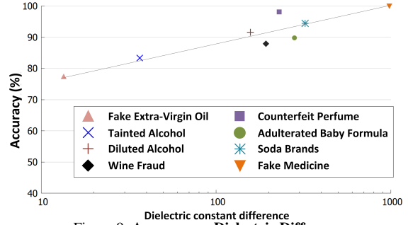
Figure 9: Accuracy vs Dielectric Differences.
