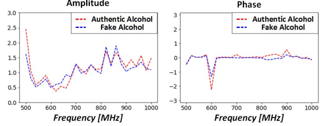
Figure 4: Output of Multipath Kernel Function.
