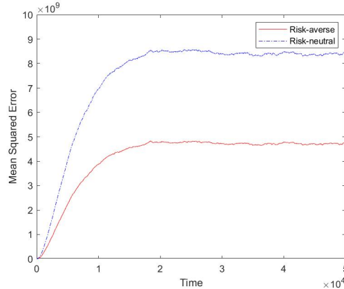
Figure 3: The mean-square errors of the policy value approximations.
