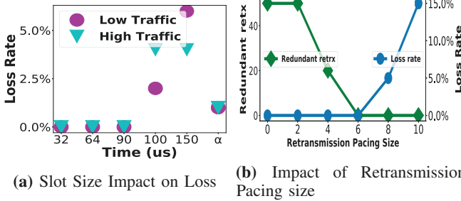
Fig. 5: (a) shows impact of DACK slot size with loss rate under environments of low (10%) and high (40%–50%) medium utilization. (b) shows larger retransmission pacing sizes lead to more losses but less redundant retransmissions, with balance at 6.
