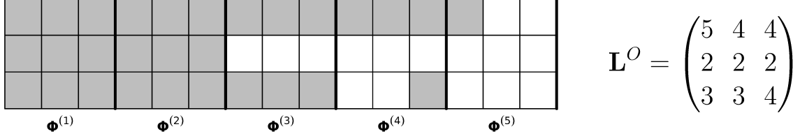
Figure 2: An own-other (O) HLa active set structure (shaded): \text{HLag}_3^O(5) .
