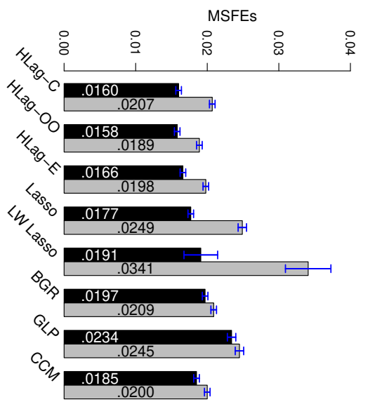
Scenario 2: Own-Other
