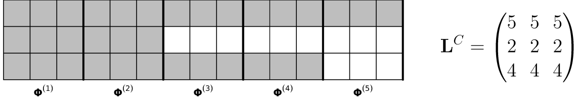
Figure 1: A componentwise (C) HLa active set structure (shaded): \text{HLag}_3^C(5) .
