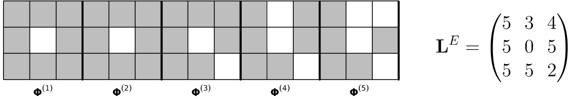
Figure 3: An elementwise (E) HLa active set structure (shaded): \text{HLag}_3^E(5) .
