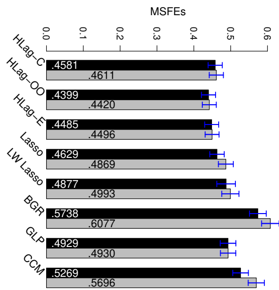
Scenario 4: Data-based
