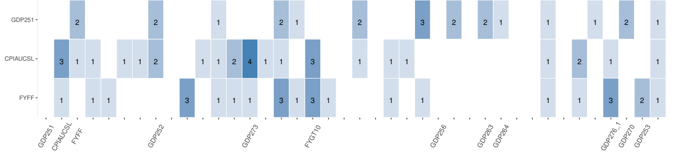
Figure 14: The first three rows of \hat{L}^E , the estimated elementwise maxlag matrix in the Medium-Large VAR for the H\text{Lag}^E method. Components with zero maxlag are left empty.
