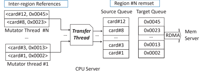
Figure 5: Semeru 's remset design; the source and target queues are implemented as bitmaps for space efficiency.
