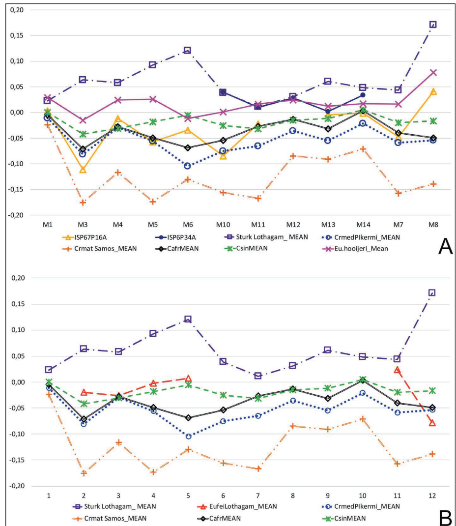
Fig. 8 - MTIII log10 ratio Diagrams. A) Metatarsal III Sahabi, European and African Hipparions, log10 ratio, Ho Std. – abbreviations as in Figure 6A. B) Metatarsal III Lothagam, European, and African Hipparions, log10 ratio, Ho. Std. Localities, as in Figure 6A.
