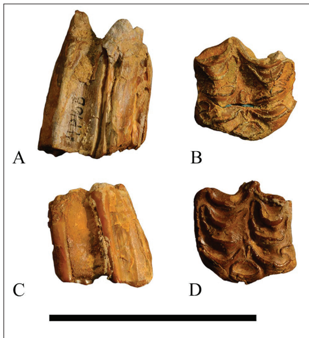
Fig. 10 - Sahabi Eurygnathohippus feibeli P3; ISP4P16B: A) labial, B) occlusal; ISP40P103A: C) labial, D) occlusal. Scale bar 5 cm.
