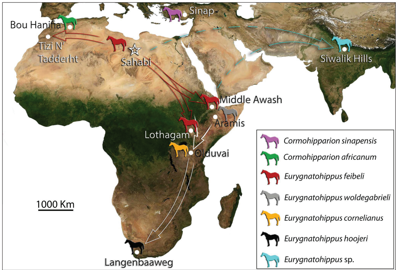
Fig. 18 - Biogeographic History of Eurygnathobippus . The genus arises from Old World Cormohippus Datum of Sinap (Turkey) Cormohippus sinapensis and Bou Hanifia (Algeria) " Cormohippus " africanum . Eurygnathobippus feibeli earliest known occurrences from Lothagam (Kenya), Sahabi (Libya), and Tizi N'Tadderht (Morocco) with slightly younger recorded occurrence from JAB Middle Awash (Ethiopia); subsequent recorded succession in East and South Africa with Eurygnathobippus woldegabrieli from Aramis (Ethiopia), Eurygnathobippus cornelianus from Olduvai (Tanzania), and Eurygnathobippus hoojeri from Langenbaaweg (South Africa).
