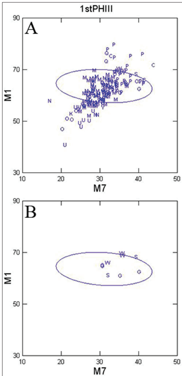
Fig. 3 - 1PHIII maximum length (M1) versus distal articular width (M7); A) entire sample; B) Lothagam (G), Sahabi (S) and Middle Awash (W) only.
