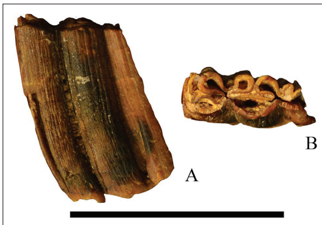
Fig. 17 - Sahabi Eurygnathohippus feibeli m3, ISP77P17A: A) labial view, B) occlusal view. Scale bar 5 cm.
