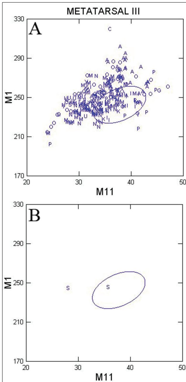
Fig. 5 - MTIII maximum length (M1) versus distal articular width (M11). A) entire sample; B) Sahabi (S) only.
