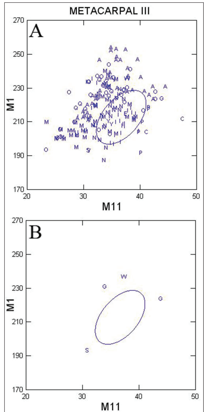
Fig. 4 - MCIII maximum length (M1) versus distal articular width (M11). A) entire sample; B) Lothagam (G), Sahabi (S) and Middle Awash (W) only.
