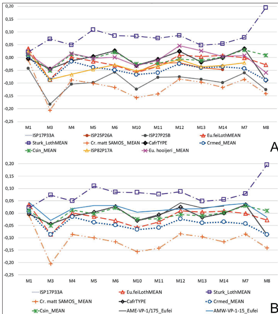
Fig. 7 - MCIH log10 ratio Diagrams. A) Metacarpal III Sahabi, Lothagam, European and African Hipparions, log10 ratio, Ho. Std. – abbreviations as in Figure 6A. B) Metacarpal III Sahabi, Lothagam, European, Middle Awash and African Hipparions, log10 ratio, Ho. Std. AME and AMW Middle Awash Localities, the remaining as in Figure 5A.
