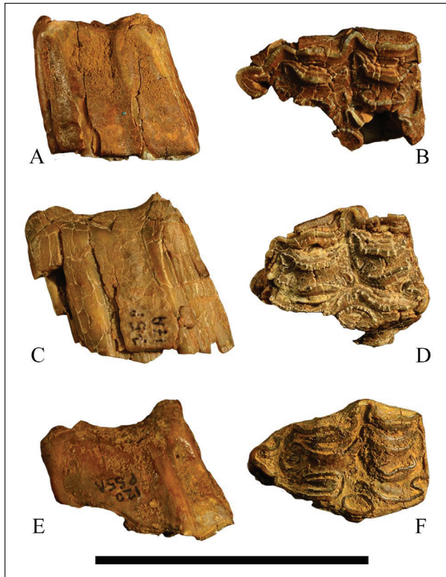
Fig. 9 - Sahabi Eurygnathohippus feibeli P2; ISP26P10A: A) labial, B) occlusal; ISP75P17A: C) labial, D) occlusal; ISP120P65A: E) labial, F) occlusal. Scale bar 5 cm.
