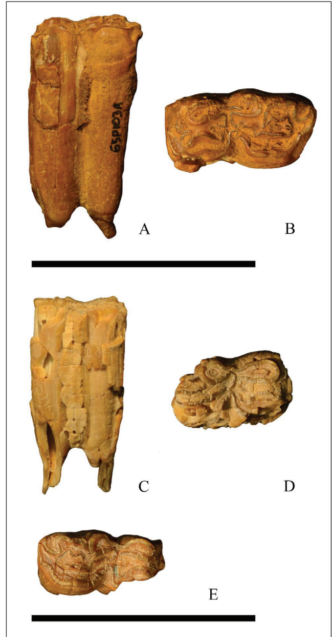
Fig. 14 - Sahabi Eurygnathobippus feibeli p4, ISP65P103A: A) labial, B) occlusal; ISP84P24: C) labial, D) occlusal; ISP183P16A: E) occlusal. Scale bar 5 cm.
