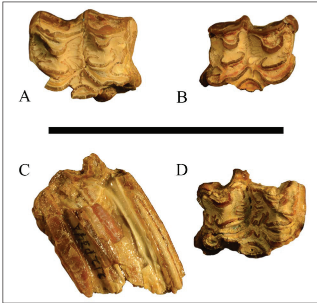
Fig. 13 - Sahabi Eurygnathobippus feibeli M3, ISP16P108A: A) occlusal; ISP63P109A, B) occlusal; ISP212P34A: C) labial, D) occlusal. Scale bar 5 cm.
