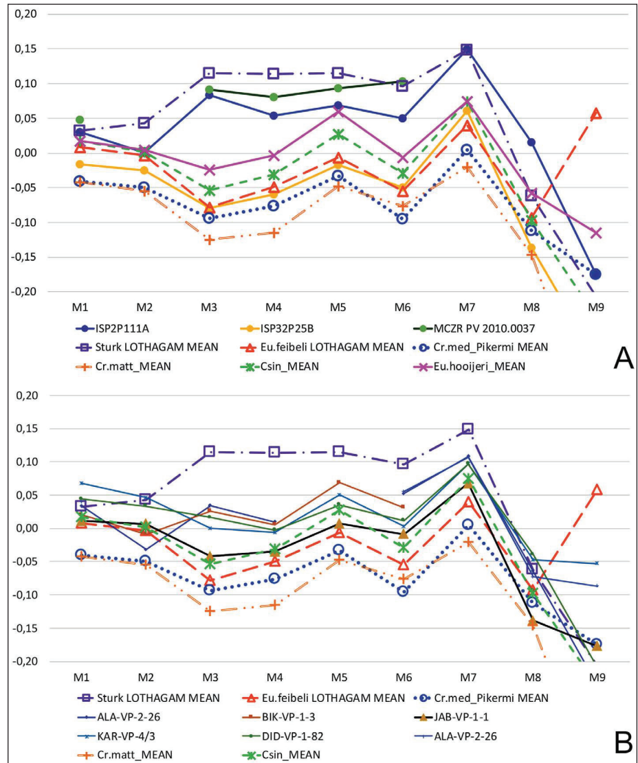
Fig. 6 - 1PHIII log10 ratio Diagrams.
