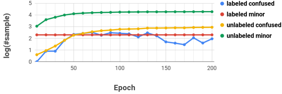
Figure 2: Number of data chosen during training.
