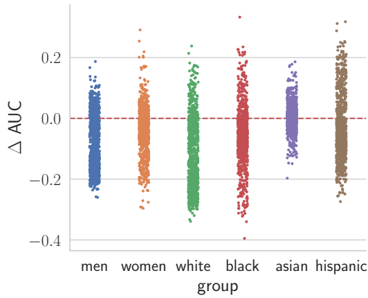
Figure 6: Differences ( \Delta s) estimated from a balanced subset of the test data with equal sample sizes for all demographic subgroups. As in Figure 3, we show deviations relative to the overall AUC for the Shock phenotype classification task.
