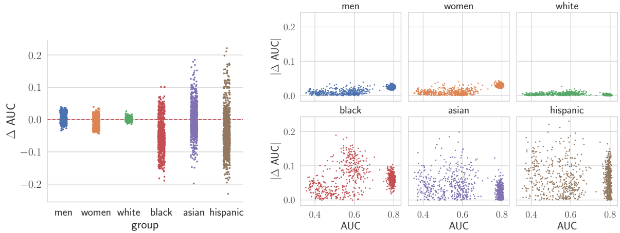
Figure 3: Differences relative to overall AUC as a function of random seeds for subgroups on the Shock phenotype classification task.
