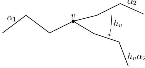
FIGURE 1. The paths \alpha and \alpha \vee_v h_v
